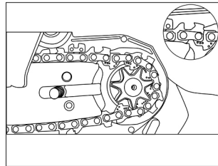
3. Place the chain around the sprocket and ensure guide bar line up the pin. Please note!!! The chain saw must be installed in the correct direction.
